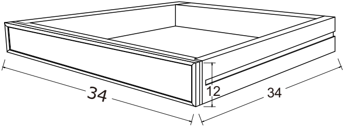
DRAWER DETAIL
