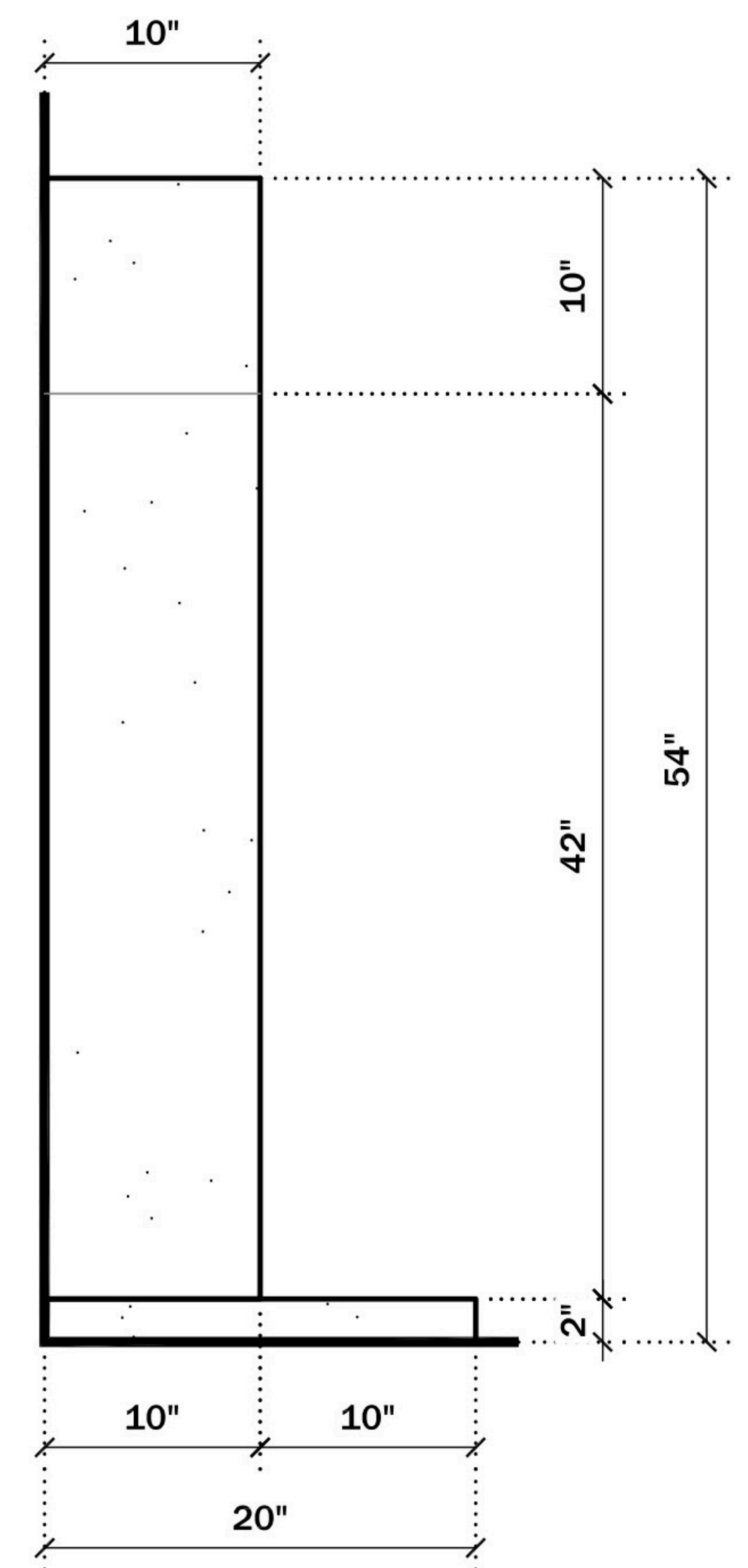
SIDE VIEW
