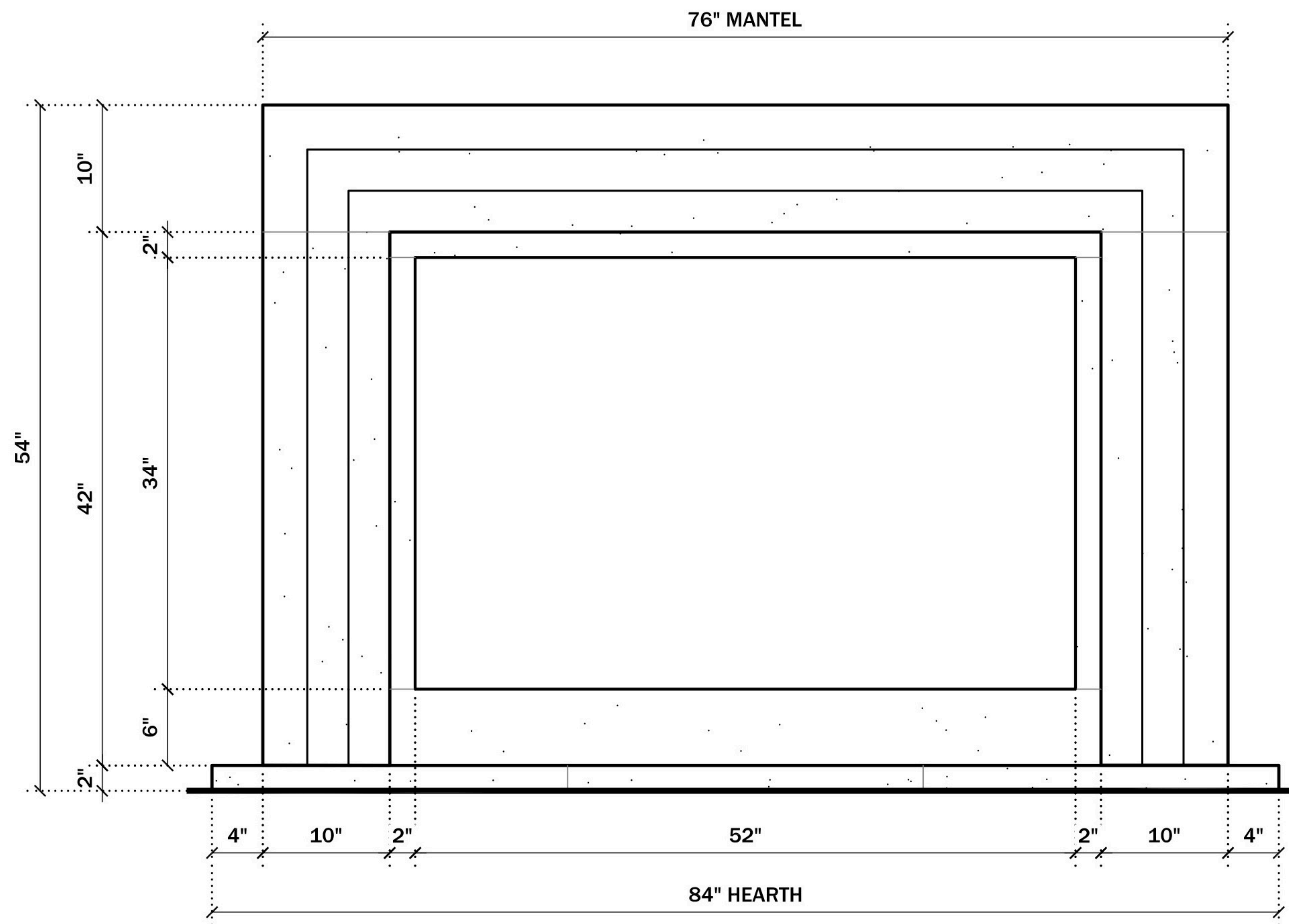
FRONT ELEVATION
