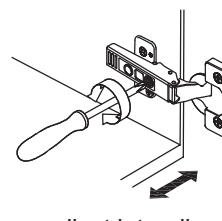
adjust laterally
