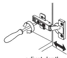
adjust depth
