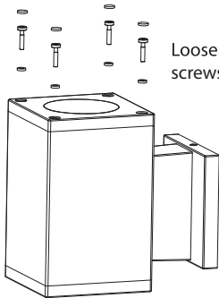
FIG.5 Loosen the fixture screws and gaskets
