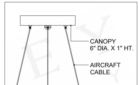
CANOPY DETAIL
