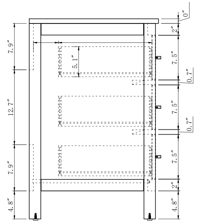
B-B SECTION
