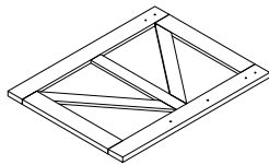
26 (507X400X14mm)X1
