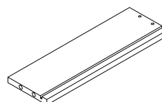
19 (300X102X12mm)X3
