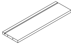
22 (339X102X12mm)X2
