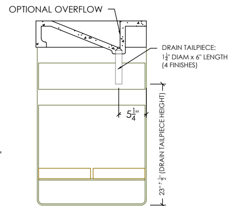
SECTION VIEW
