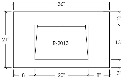
FRONT ELEVATION
