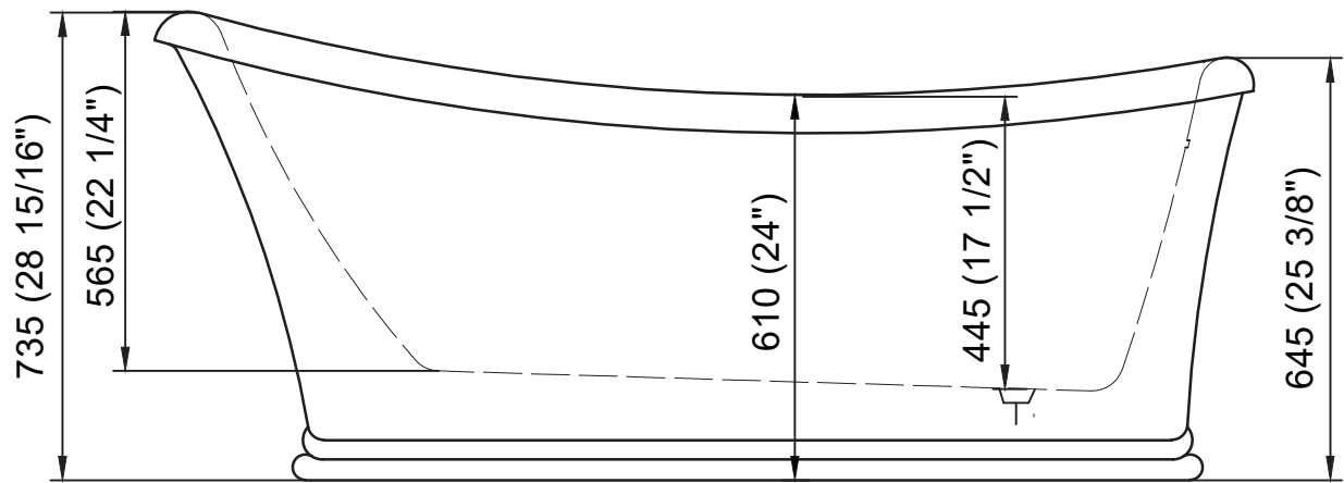
Side
