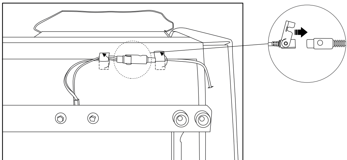
BOTTOM VIEW
