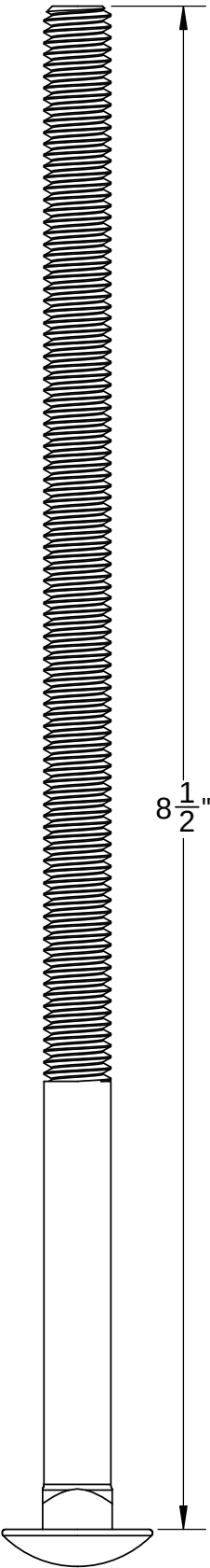
3/8" X 8-1/2" CARRIAGE BOLT QTY: 1
