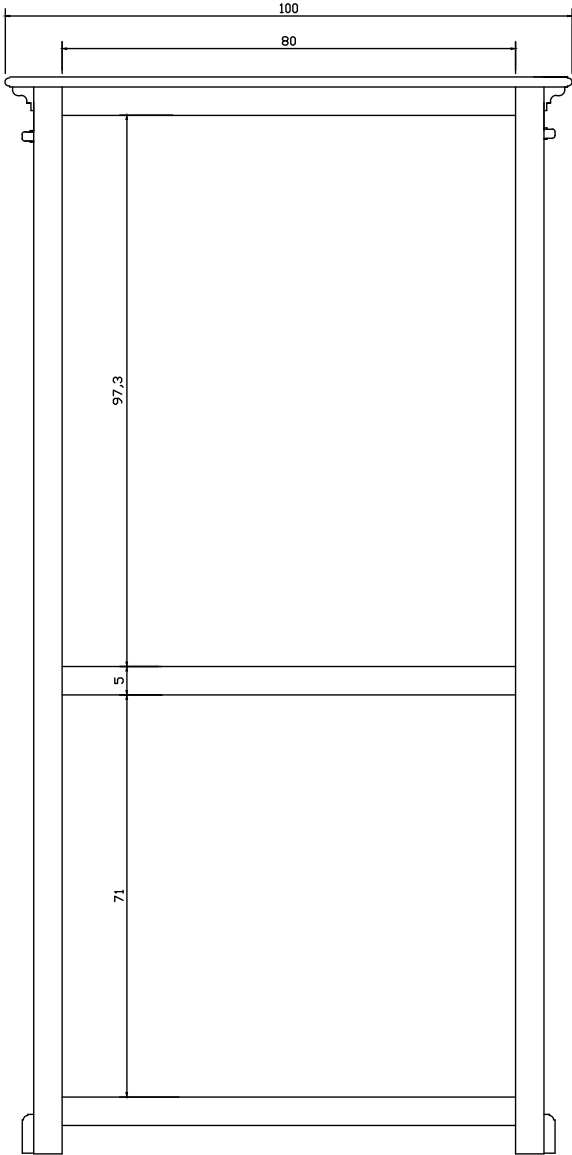
BACK VIEW
