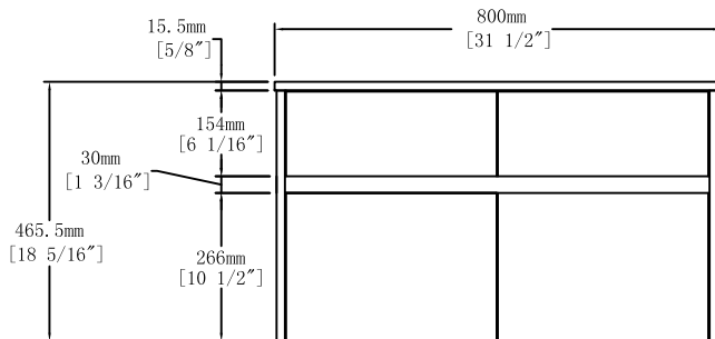
Front View
