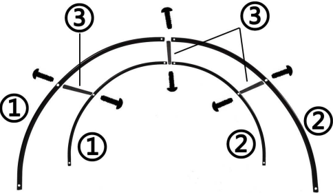
Step 1. Assemble the top.
