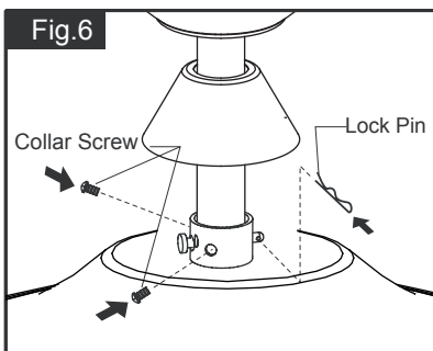
Fig.6 Insert and tighten the two Collar Screws. Slide Lock Pin into Hanger Pin until it is locked into position.
