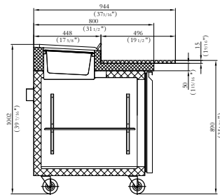
SECTION VIEW
