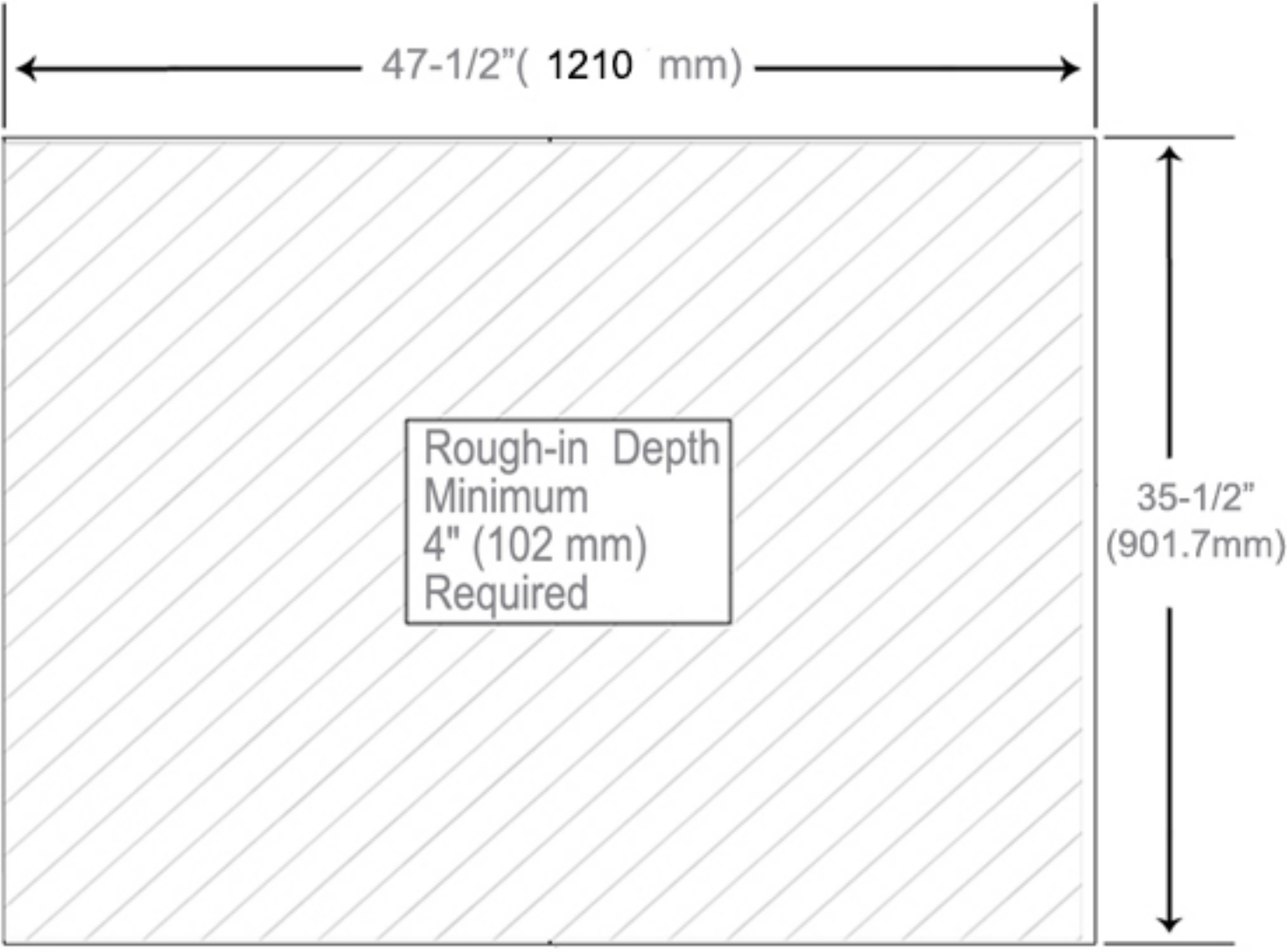
Rough-in Dimensions
