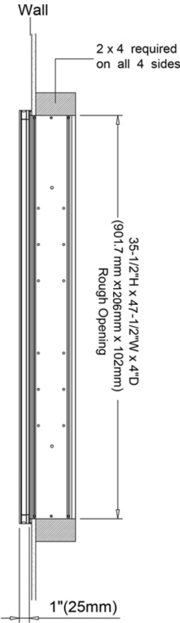
Recessed Mount
