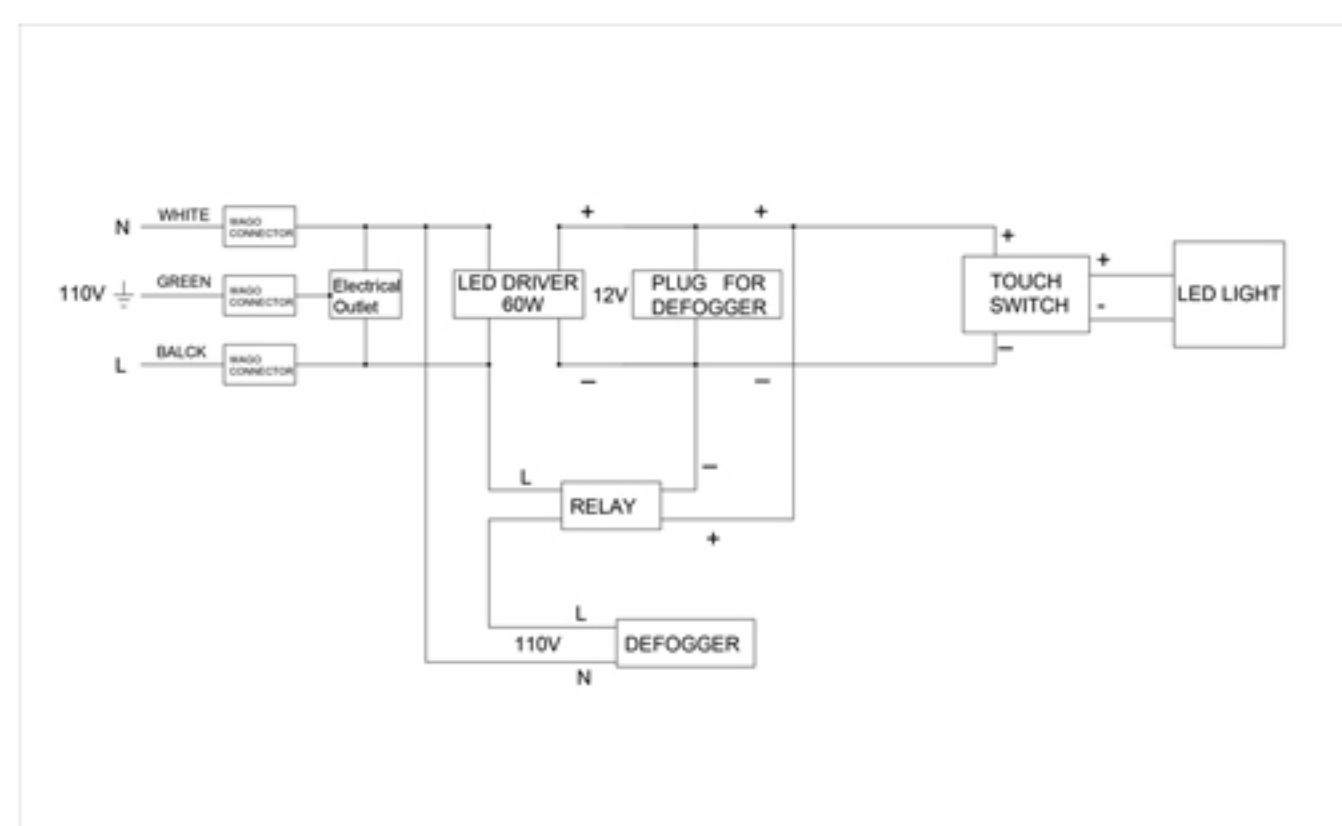
Circuit Diagram
