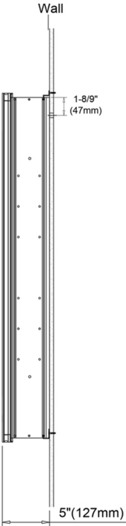
Surface Mount
