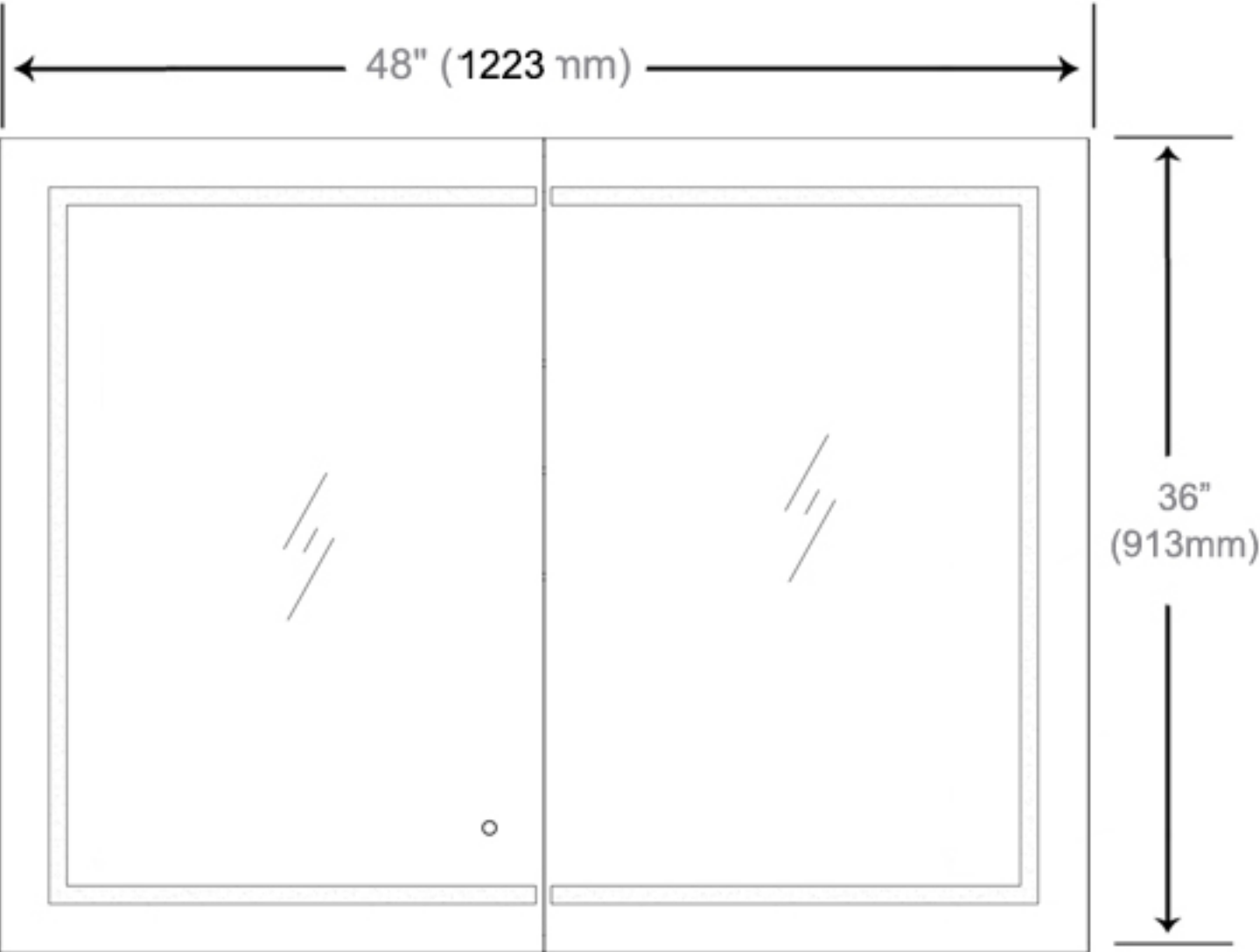
Cabinet Dimensions
