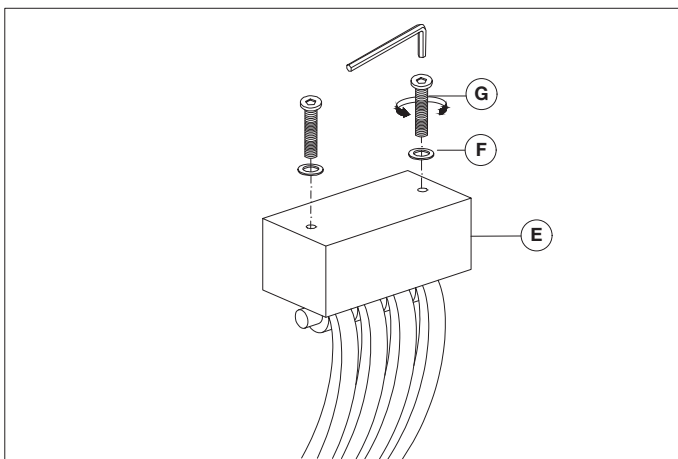
2. Assemble the marble base to the frame.
