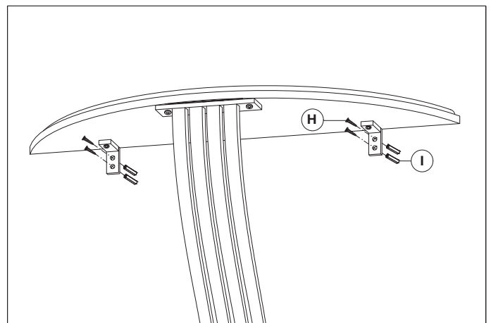
4. Mount the table to the wall.
