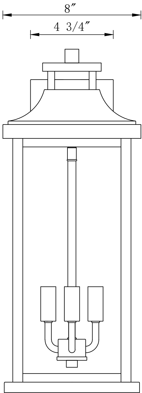
FRONT VIEW
