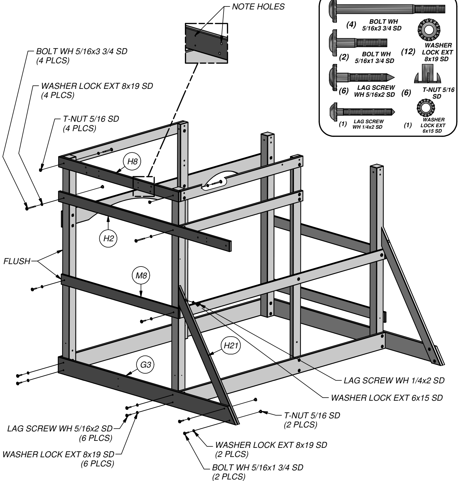
(1) H21 - ANGLE BRACE - W4L11112 1"x3 3/8"x47 1/4" (24x86x1201)
