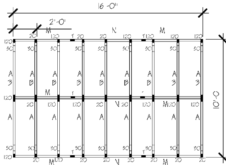
ROOF PLAN
