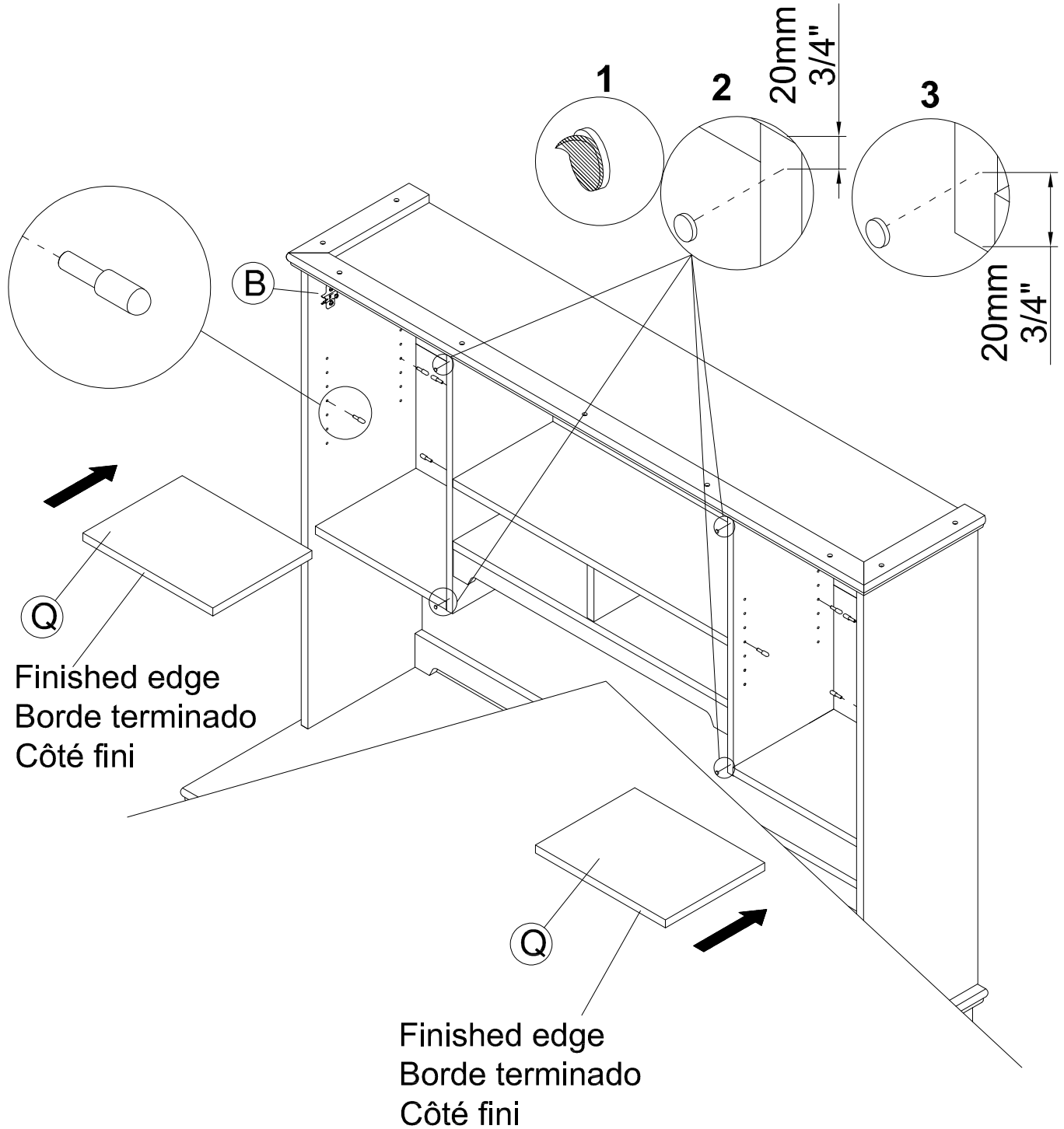
Shelf Pin
