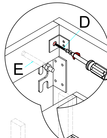
Screw (D): M5 x 50mm long (2pcs)
