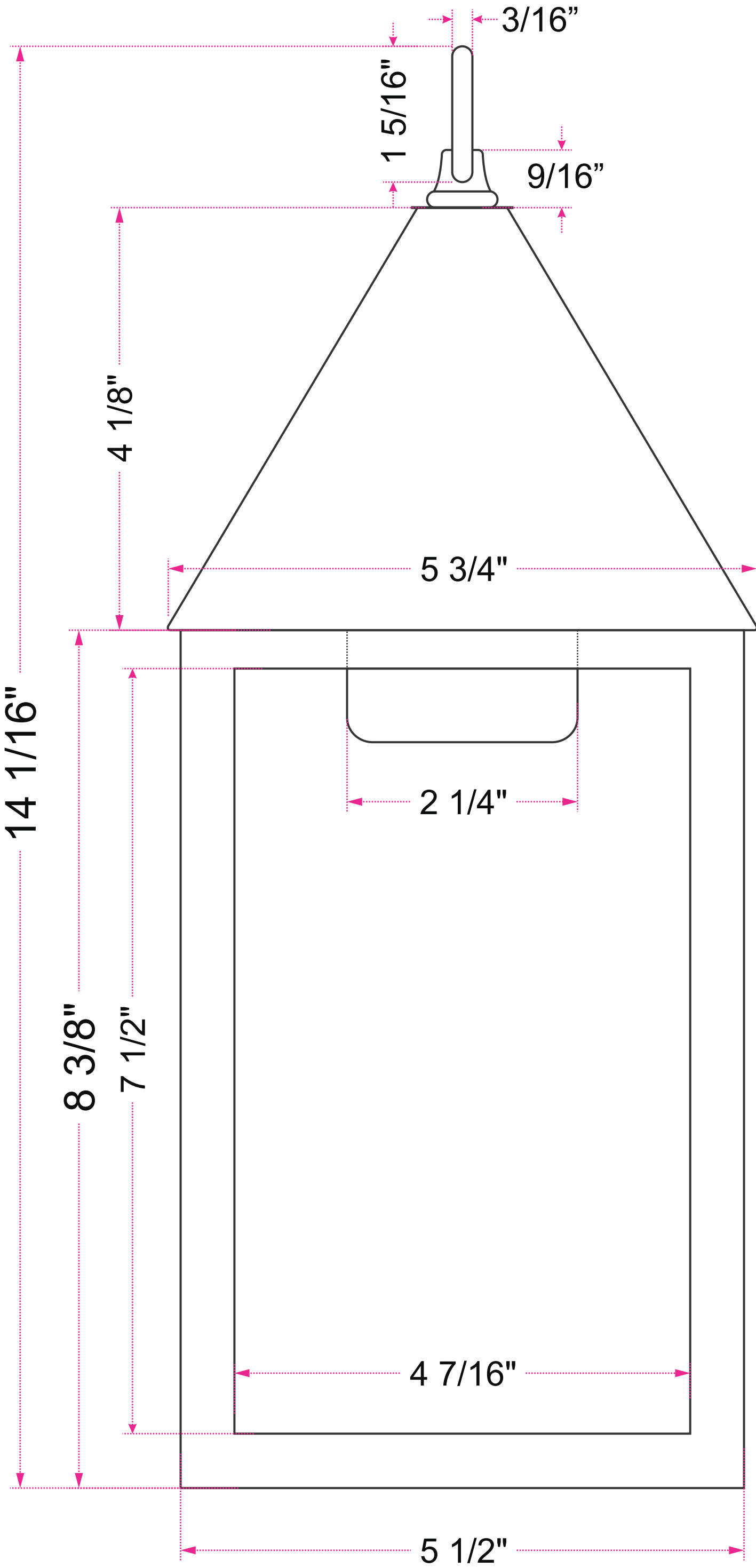
Side View
