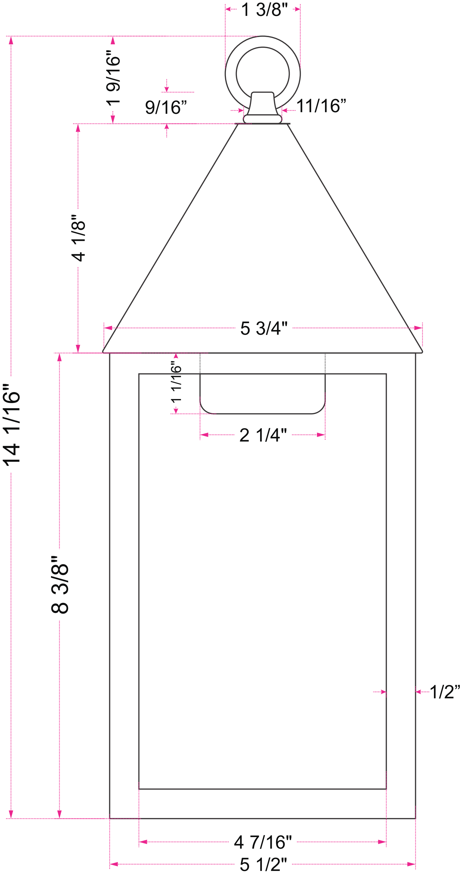
Front View
