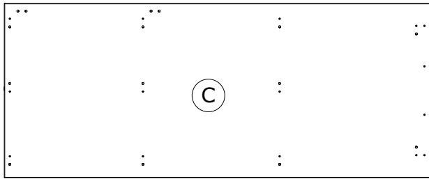
CA3591 1700x690x38mm
