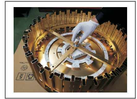
Step 5. Fasten the decorative accessories to the screw. As is shown in the figure.
