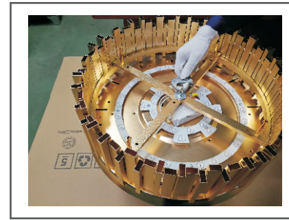
Step 4. The hole in the middle of the lampshade corresponds to the screw in the middle of the chassis. Fix it with nuts and gaskets and tighten it with tools.
