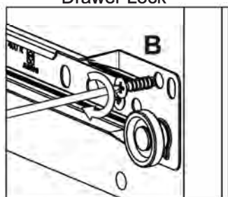
Detail 16 Drawer Lock
