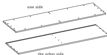
Bottom Panel
