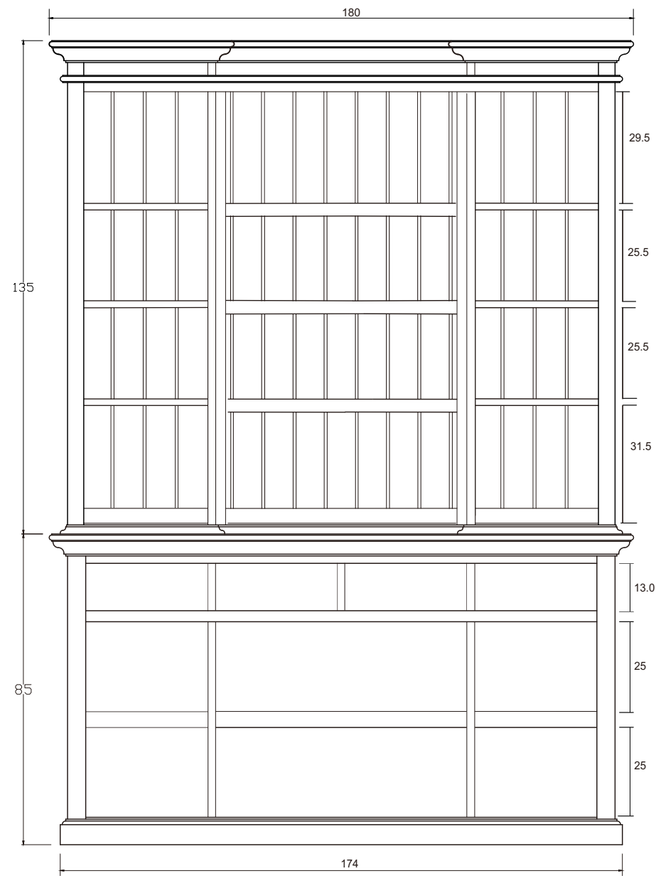
FRONT OPEN
