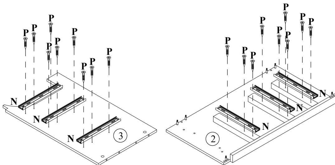
POSITION OF SCSEW
