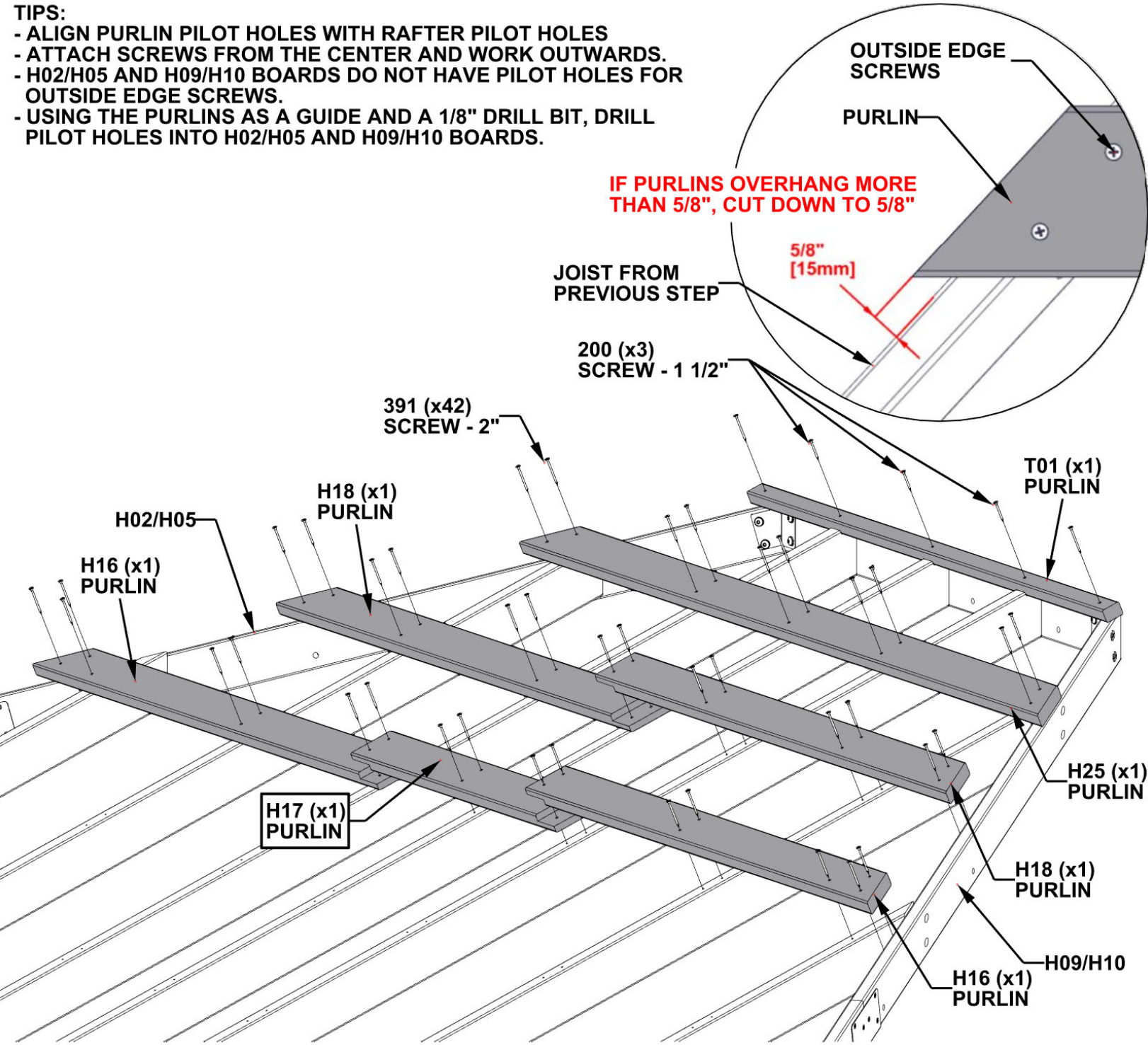
H25 | PURLIN - W4L15308 (1) 1"x3 3/8"x75 1/16" (24x86x1907)
