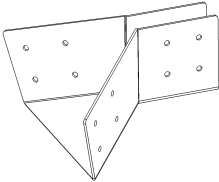
A4M01184 | PANEL SUPPORT BRACKET (2)
