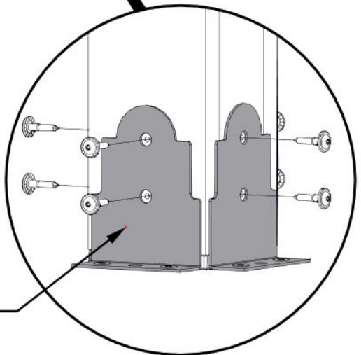
1793 (x8) STEEL POST ACHOR PLATE
