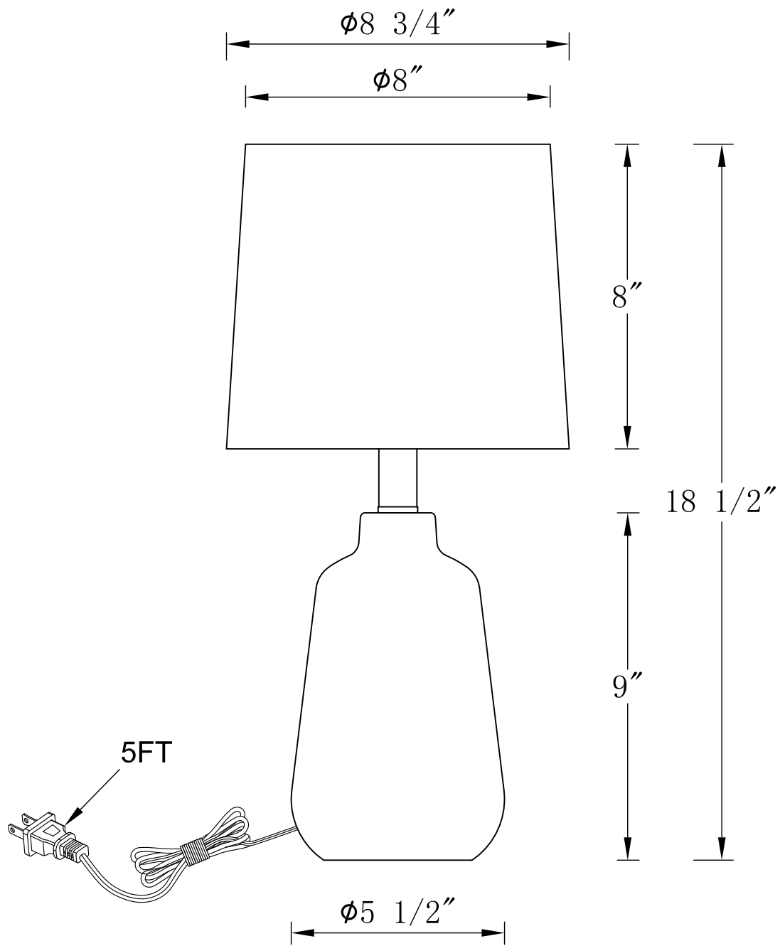
FRONT VIEW
