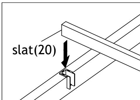
3. Put the slat (20) into the clamp.
