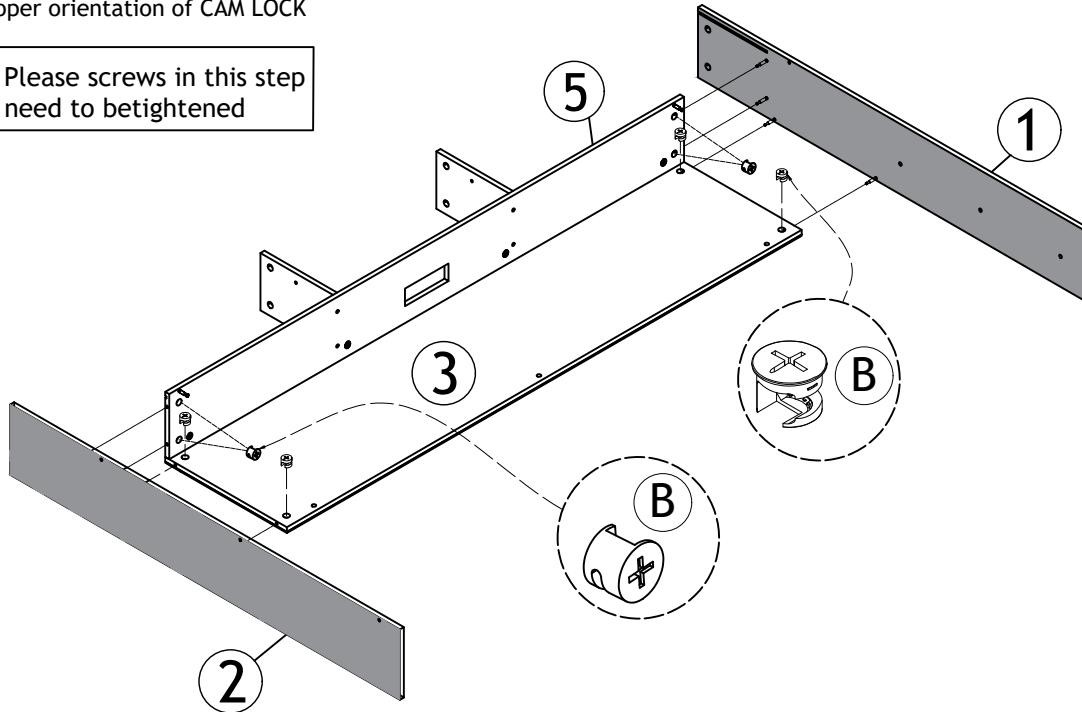
Proper orientation of CAM LOCK
