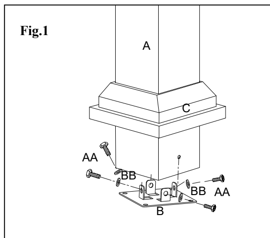
Fig.1: Insert Base Cover (C) into Post (A), then fixed Base (B) to bottom of Post (A) by bolt (AA) and Washer (BB)
