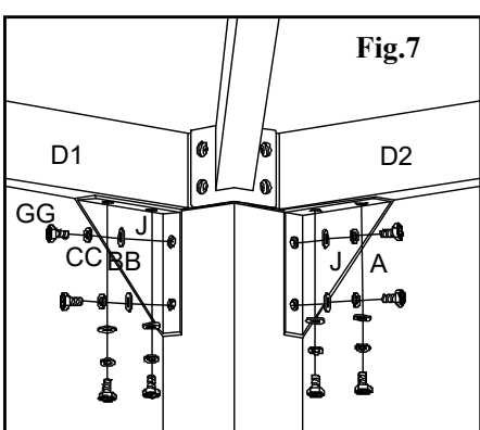
Fig.7: Attached Corner Support (J) to Post (A) and Cross Beam1/2 (D1/2) by Bolt (GG), Spring Washer (CC) and Washer (BB). Plea.
