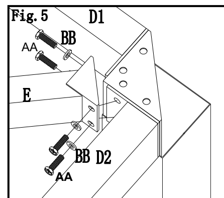
Fig.5: Fix the assembled inclined beam(E) to the column with bolt (AA), washer(BB) and corss beam(D1、D2)
