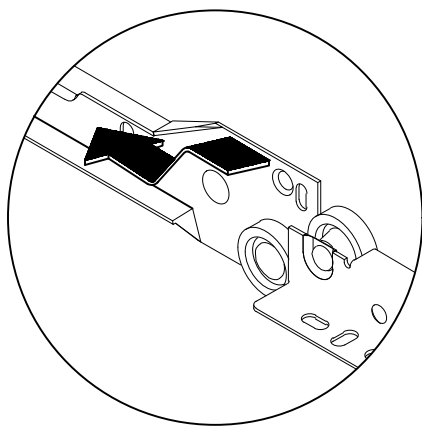
Drawer Slide
