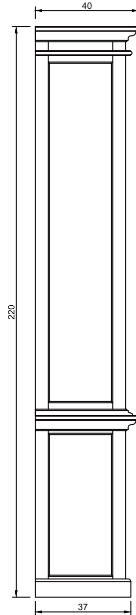
SIDE VIEW
