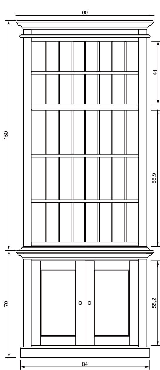
FRONT VIEW
