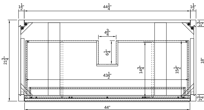
TOP VIEW OF VANITY CABINET
