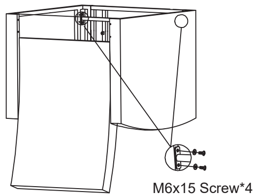
Step 6 (Using rubber ring)
