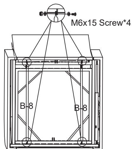
Step 6 (Using rubber ring)
