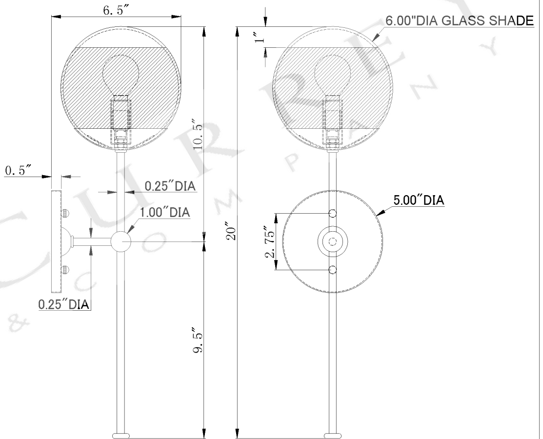
SIDE VIEW
