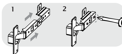
Inset Hinge
