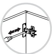
/ LATERAL ADJUSTMENT
