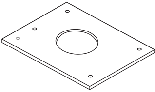
B-520X440mm(1pc)
