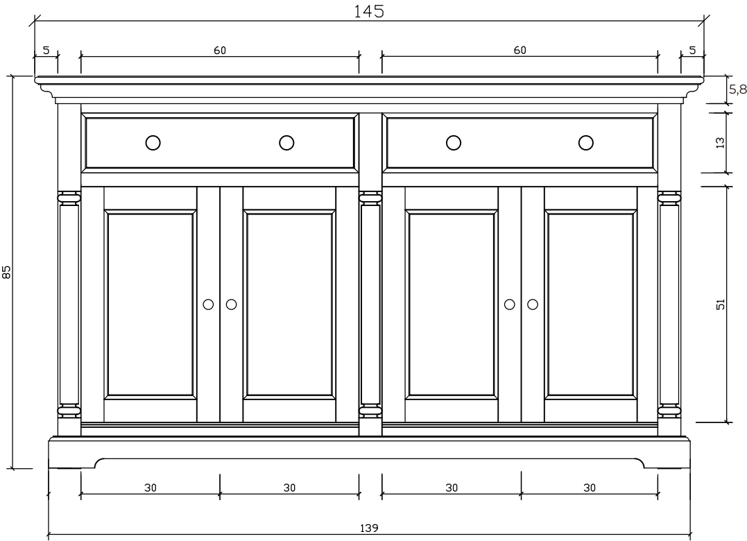
FRONT VIEW
