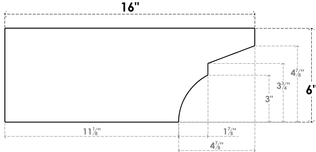
SIDE PROFILE
