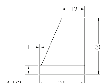
48" SIDE VIEW
