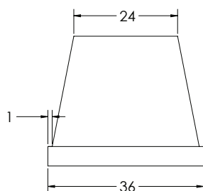
36" FRONT VIEW
