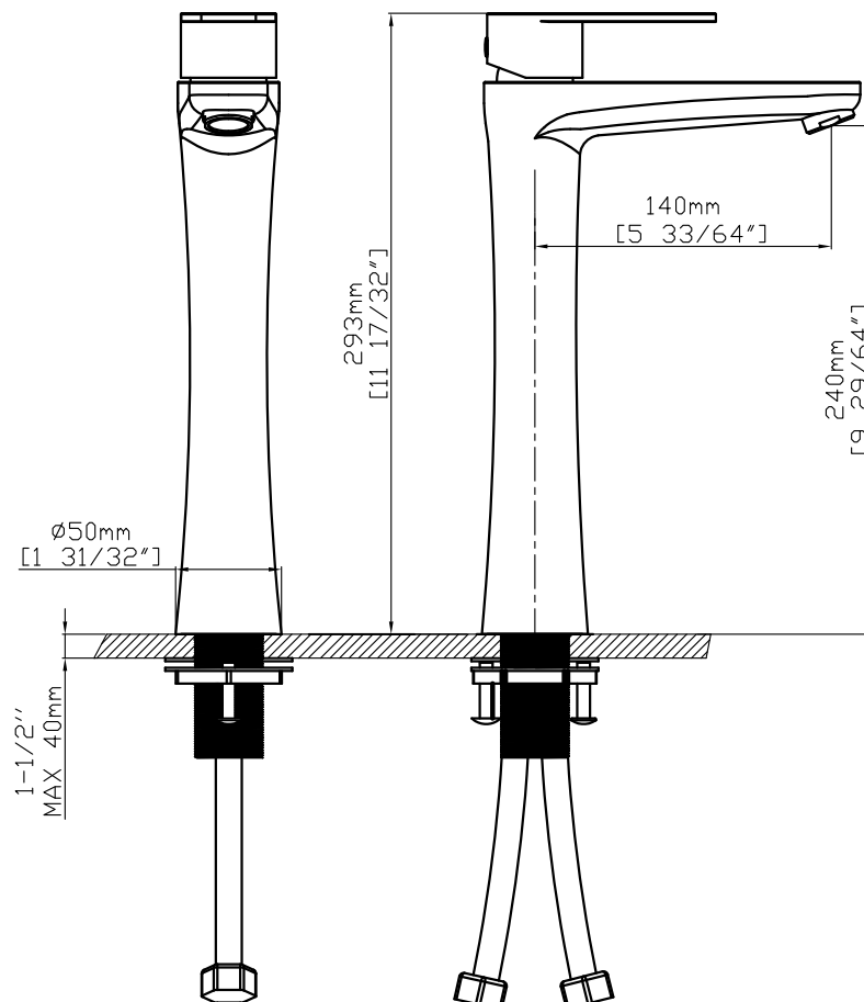
CRITICAL DIMENSIONS
