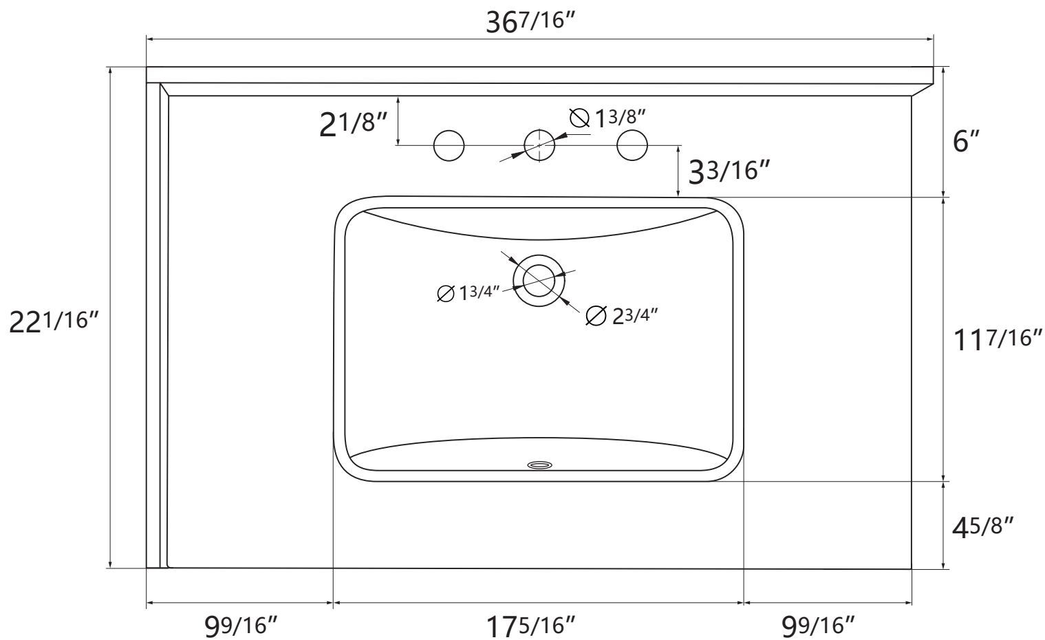
Top View
