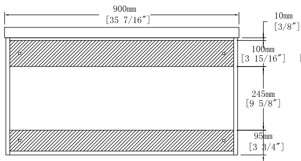
Back View
