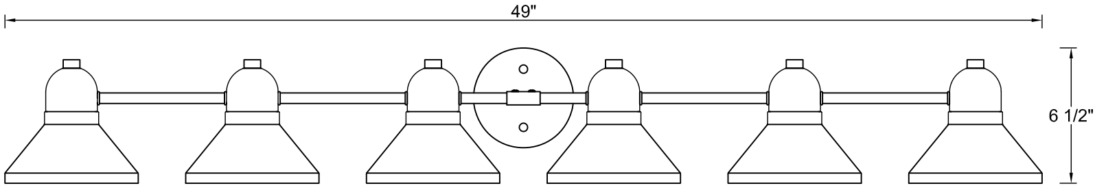
FRONT VIEW
