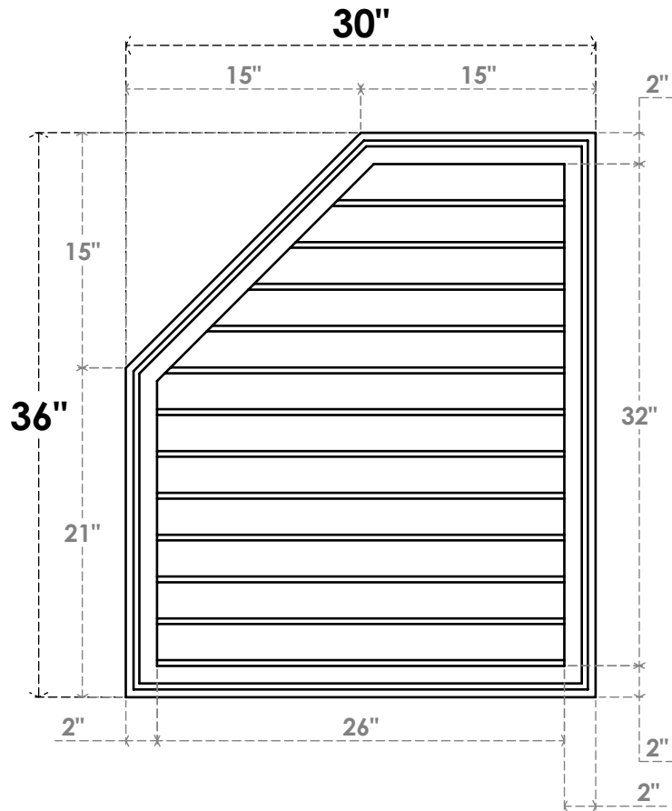
FRONT
