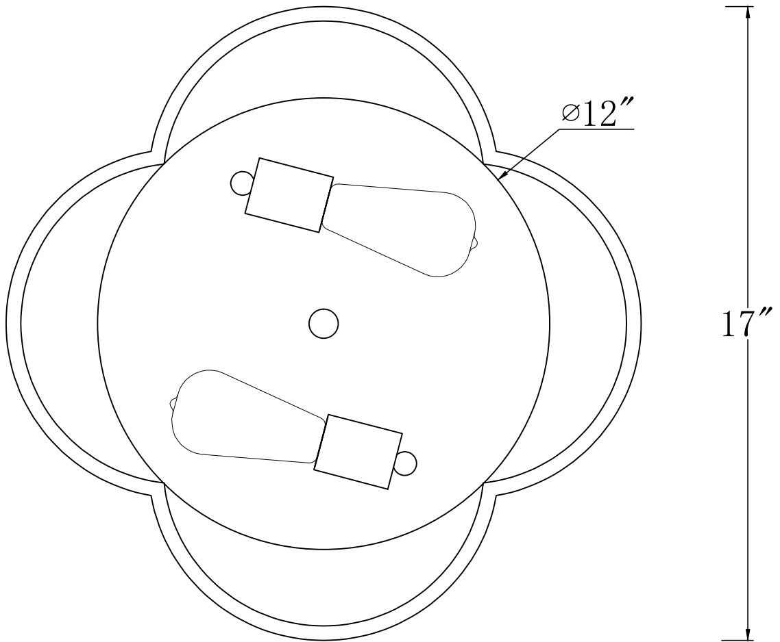
TOP VIEW
